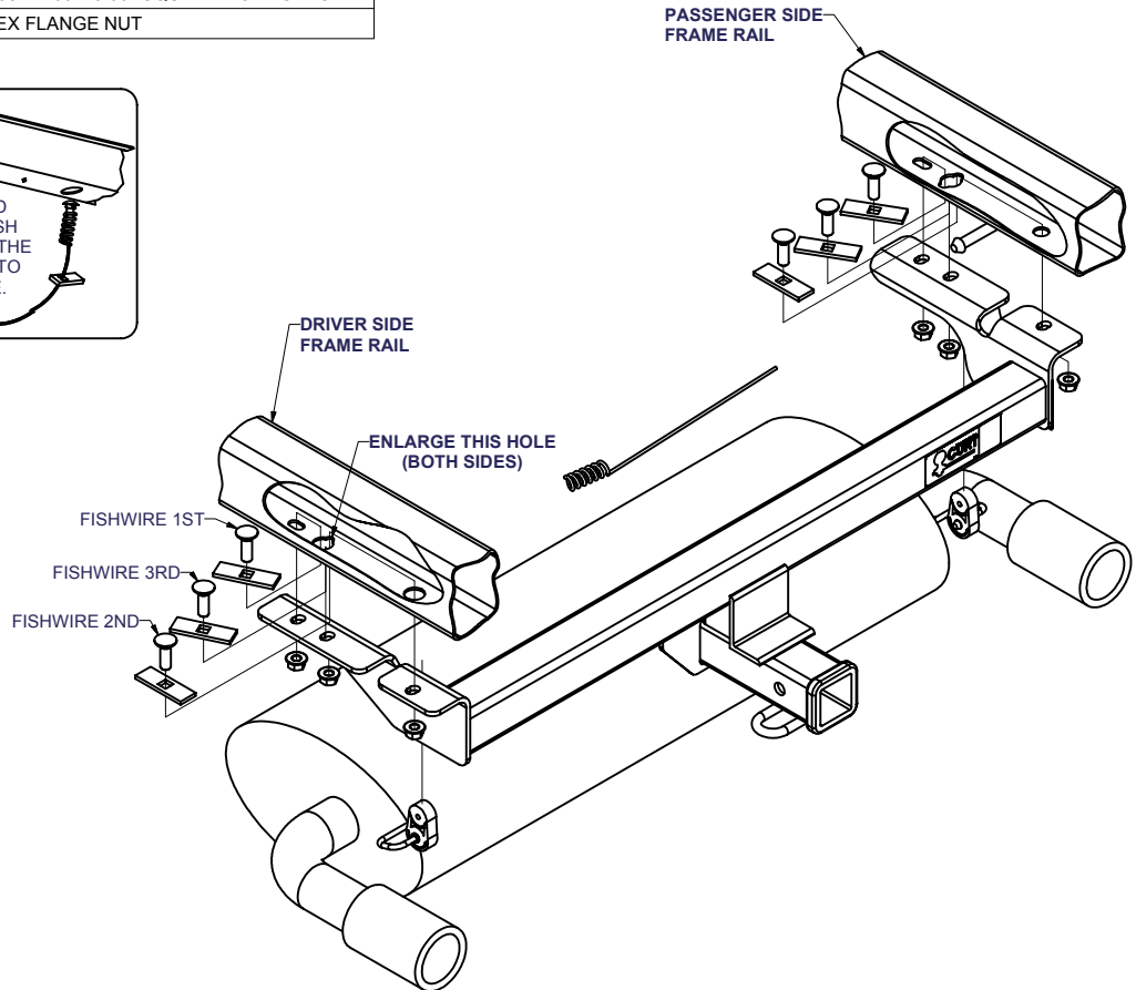
CENTER HOLE ENLARGEMENT DIAGRAM
