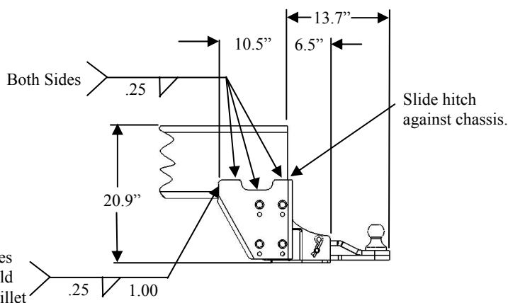
DRIVERS SIDE OF CHASSIS LOOKING AT THE PASSENGER SIDE
