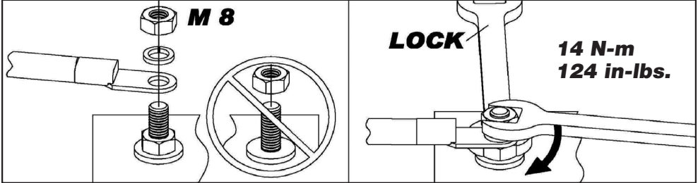
Figure 2 - Torque Specification
