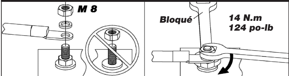
Figure 2 - Couples de serrage
