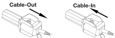
Figure 5 - Cable Button
