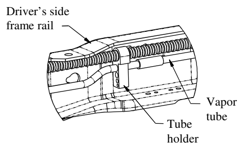
Figure 1a Inside of frame rail
