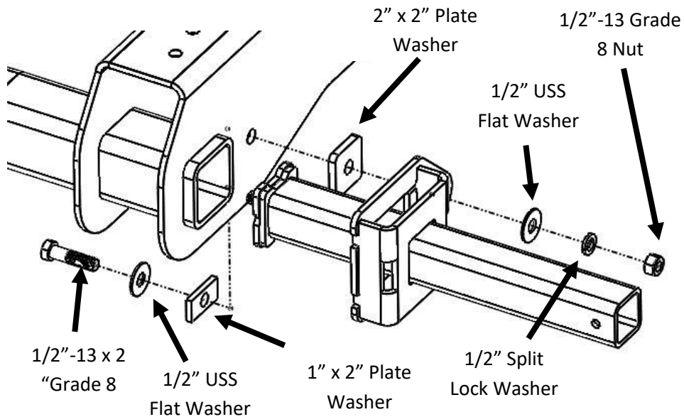
Figure 2.1 (Passenger Side Shown with F-250 Hitch Adapter Shown)
