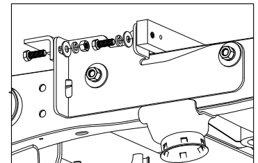
FIGURE C11: View from outside of Driver Side Frame
