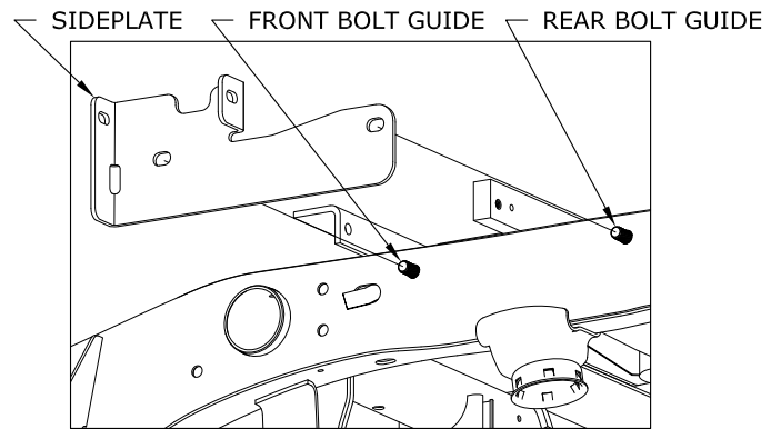
FIGURE C9: View from outside of Driver Side Frame
