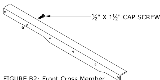
FIGURE B2: Front Cross Member
