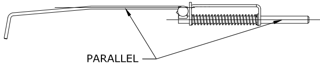
FIGURE E2: Latch Assembly
