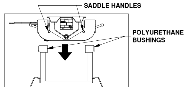
FIGURE D1: View of coupler and base. (Saddle Handles up)
